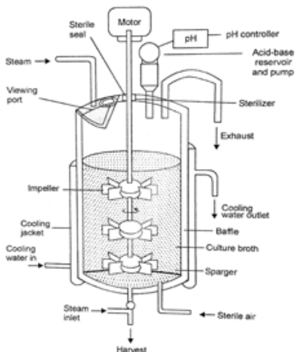
Fig Basic design of a fermentor (Bioreactor)
